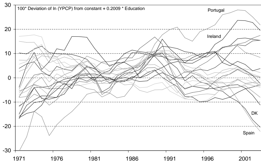
Figure 2: Errors from cointegration between GDP and years of education
